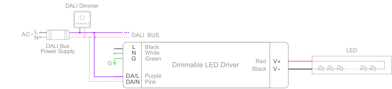
Diagram 1 DALI Dim
