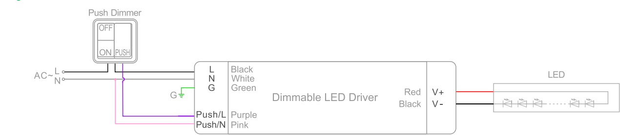
Diagram 2 Push-Dim
